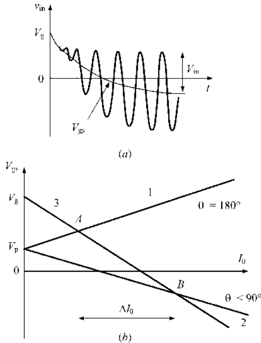
FIGURE 8.17 Self-bias operation.
