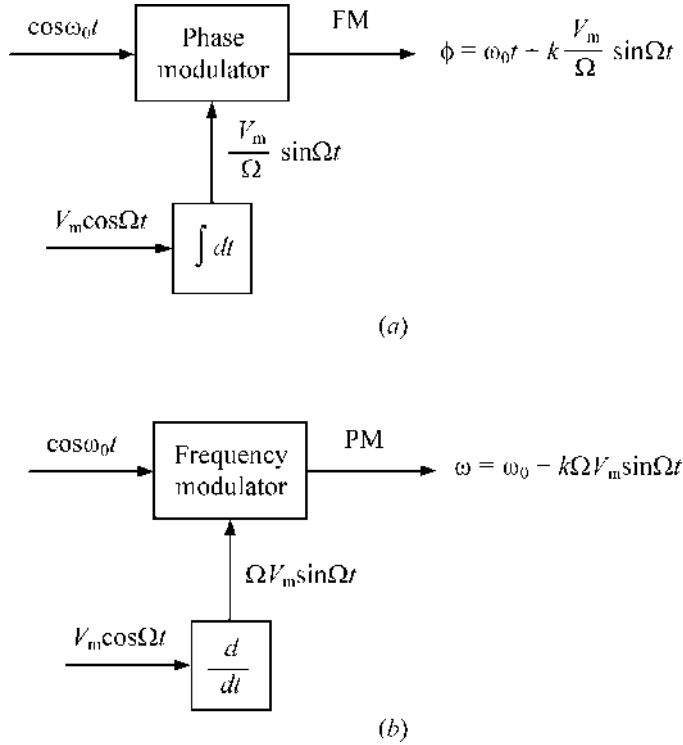
FIGURE 6.24 Indirect methods of frequency and phase modulations.
