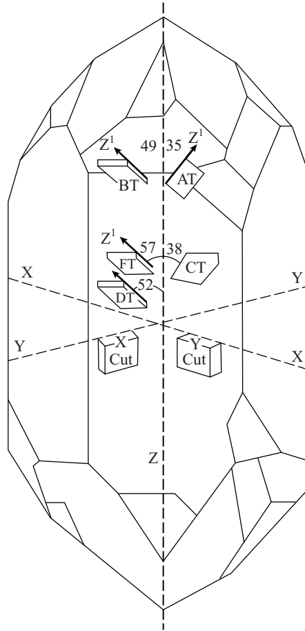
FIGURE 8.59 Typical crystal cuts from a doubly terminated quartz crystal.
