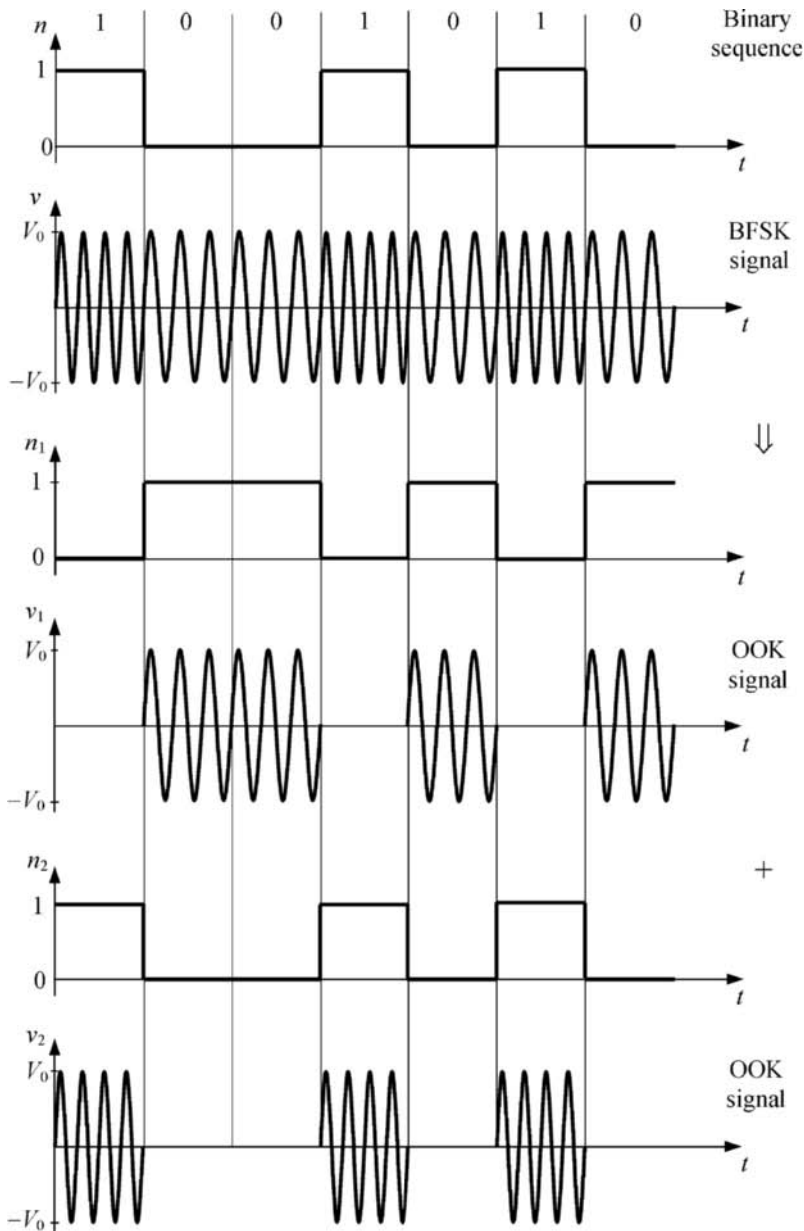
FIGURE 6.33 BFSK signal as sum of two OOK signals.
