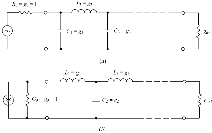
FIGURE 5.11 Ladder circuits for low-pass filter prototypes.
