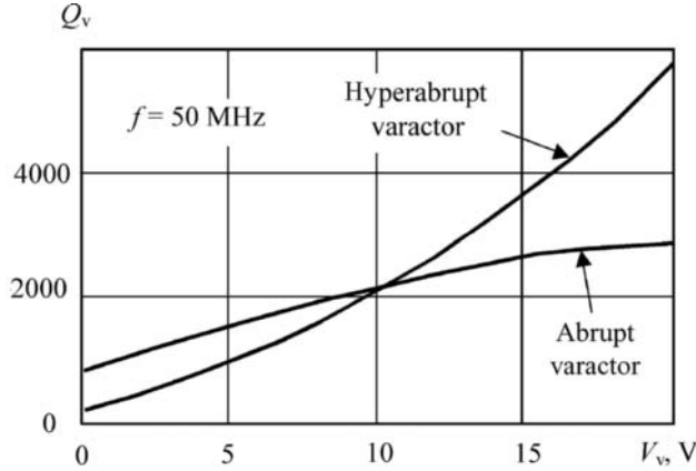
FIGURE 2.7 Varactor quality factor versus bias voltage.
