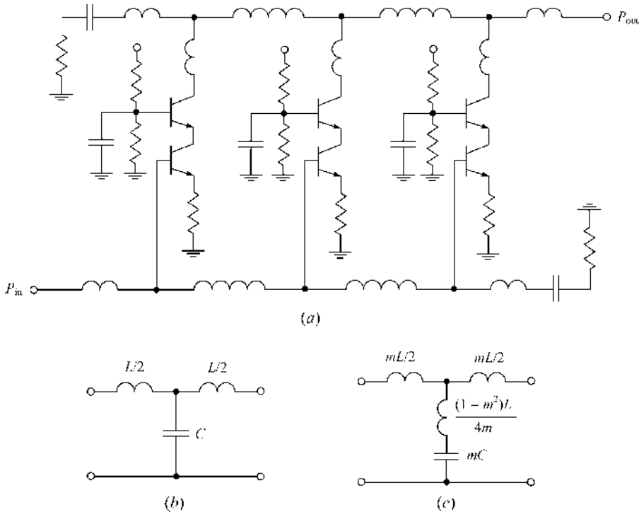
FIGURE 10.60 Schematic of three-stage bipolar cascode distributed amplifier.
