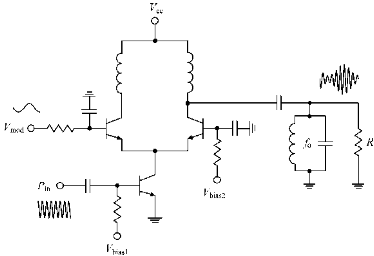
FIGURE 6.6 Collector modulation using differential pair.
