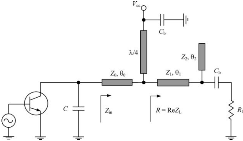
FIGURE 11.54 Schematic of transmission-line Class E power amplifier.
