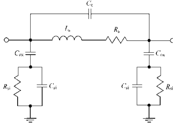
FIGURE 1.12 Equivalent circuit of a square spiral inductor.
