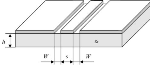
FIGURE 1.24 Coplanar waveguide structure.
