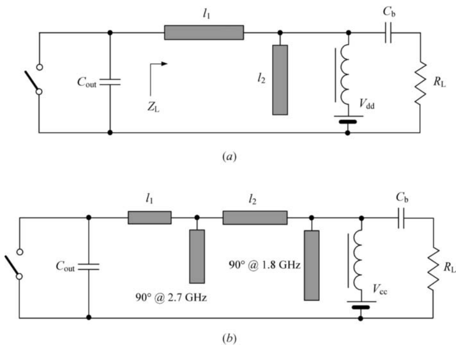
FIGURE 11.35 Equivalent circuits of Class E power amplifiers with transmission lines.
