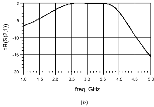
FIGURE 10.44 Two-section broadband low-pass matching circuit and its frequency response.
