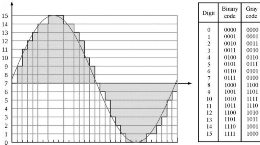
FIGURE 6.44 Signal sampling and quantization for 4-bit PCM.
