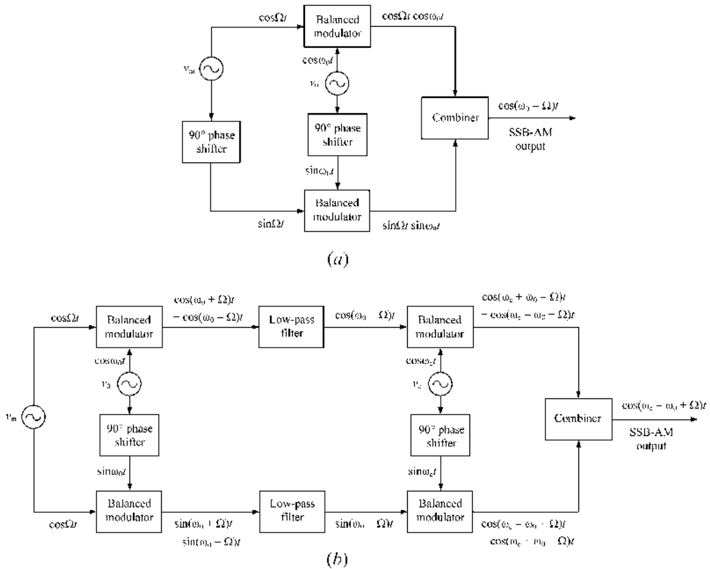
FIGURE 6.10 Methods of single-sideband modulation.
