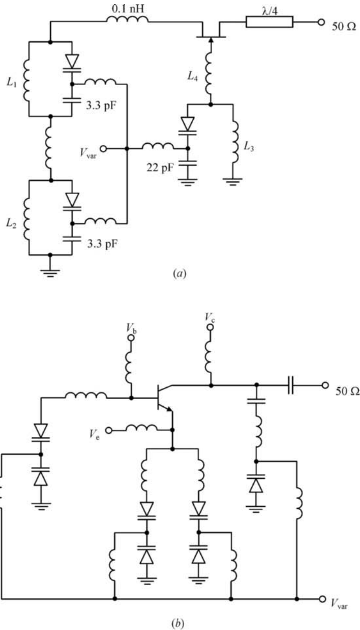
FIGURE 14.30 Microwave monolithic very wideband VCO circuits.
