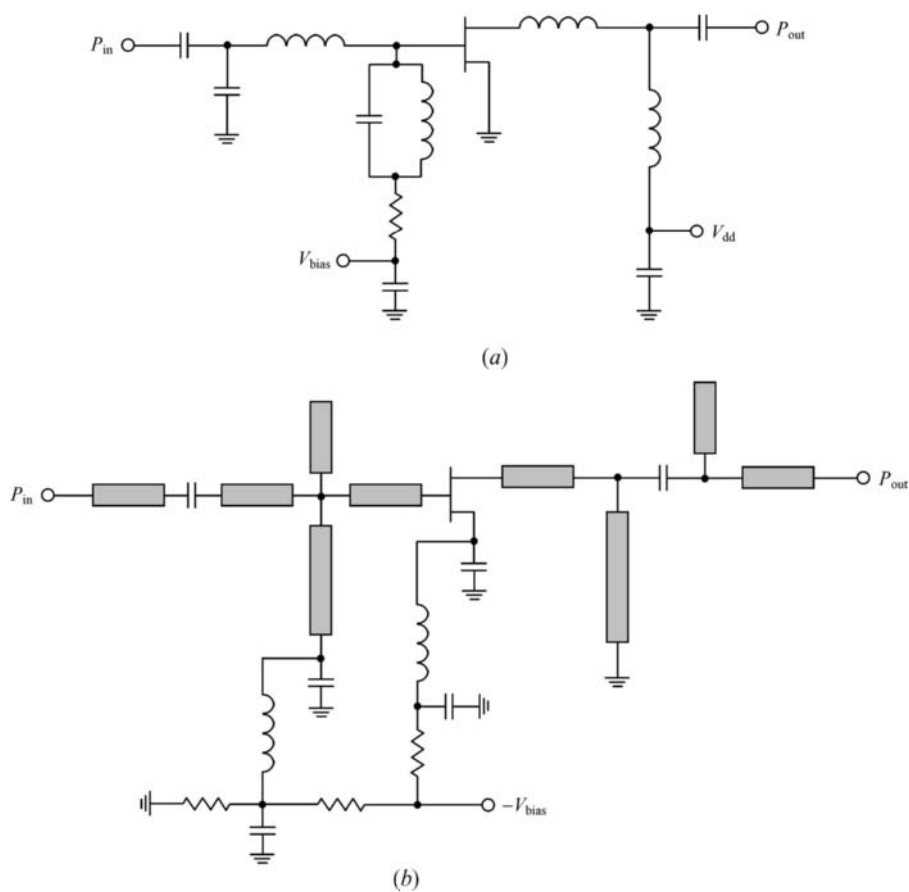
FIGURE 13.32 Schematics of MESFET limiters.
