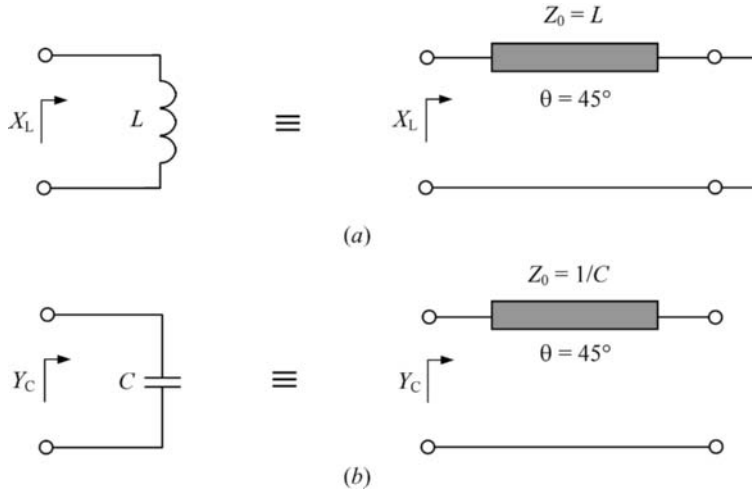
FIGURE 5.19 Equivalence between lumped elements and transmission lines.
