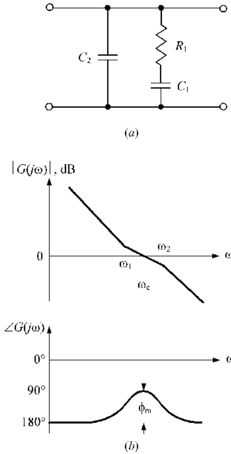
FIGURE 9.16 Passive filter for third-order loop and Bode plot.
