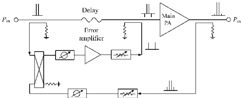
FIGURE 12.16 Power amplifier module with feedback-feedforward linearization.
