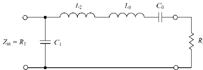
FIGURE 3.11 L -transformer with additional LC -filter.
