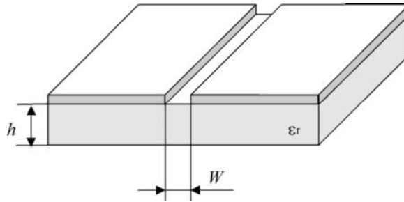
FIGURE 1.22 Slotline structure.
