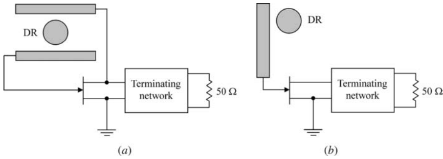
FIGURE 8.68 Schematics of dielectric resonator oscillator.
