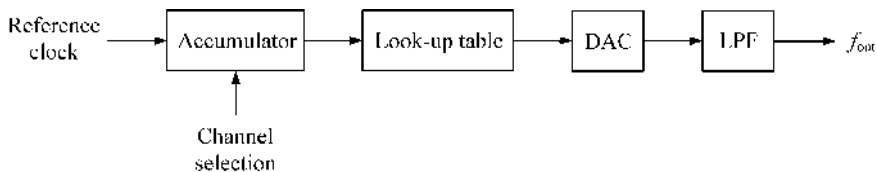
FIGURE 9.34 Block diagram of direct digital synthesizer.
