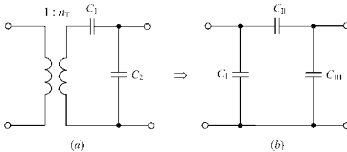
FIGURE 10.41 Capacitive impedance-transforming circuits.
