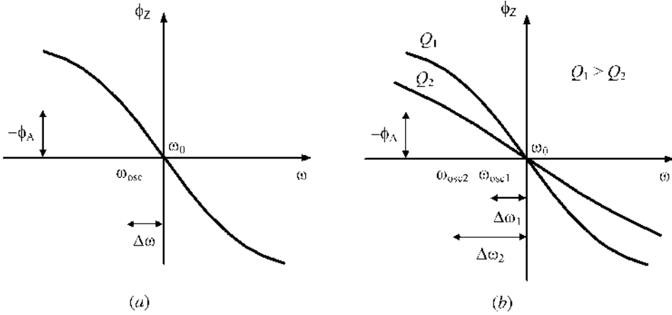
FIGURE 8.3 Deviation of oscillation frequency f_{osc} from resonant frequency f_0 .
