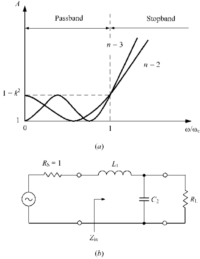
FIGURE 5.12 Equal-ripple responses and low-pass filter prototype.
