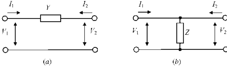
FIGURE 1.6 Single-element networks.
