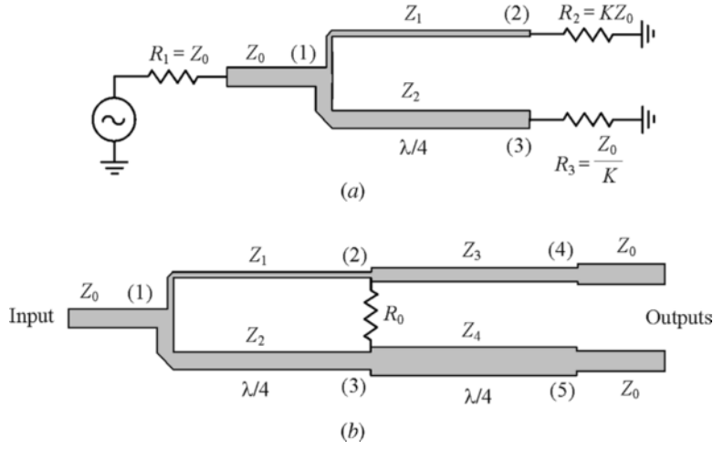
FIGURE 4.28 Split-tee power divider.
