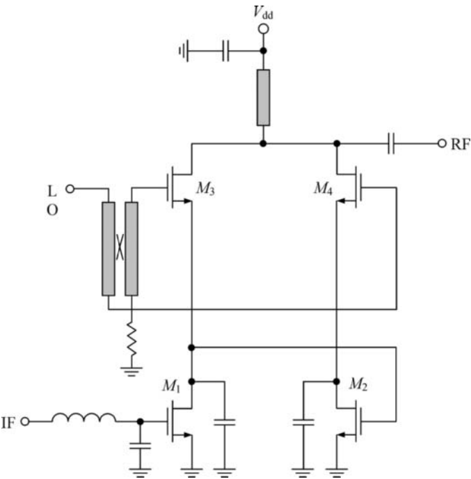
FIGURE 7.17 Schematic of balanced CMOS upconversion mixer MMIC.
