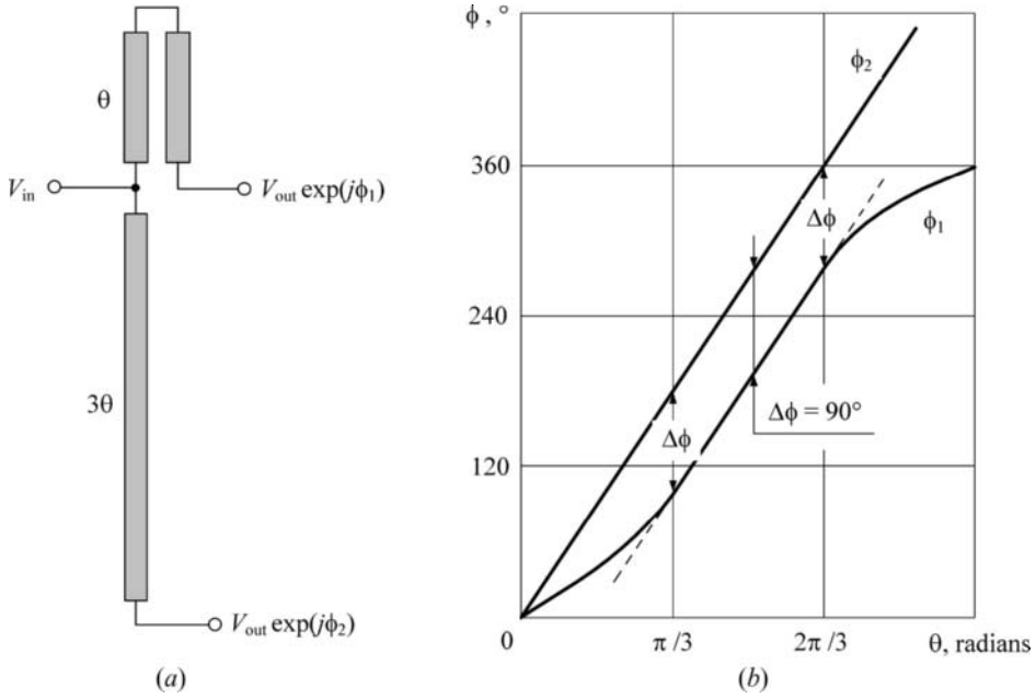
FIGURE 13.18 Schiffman differential 90^\circ phase shifter.
