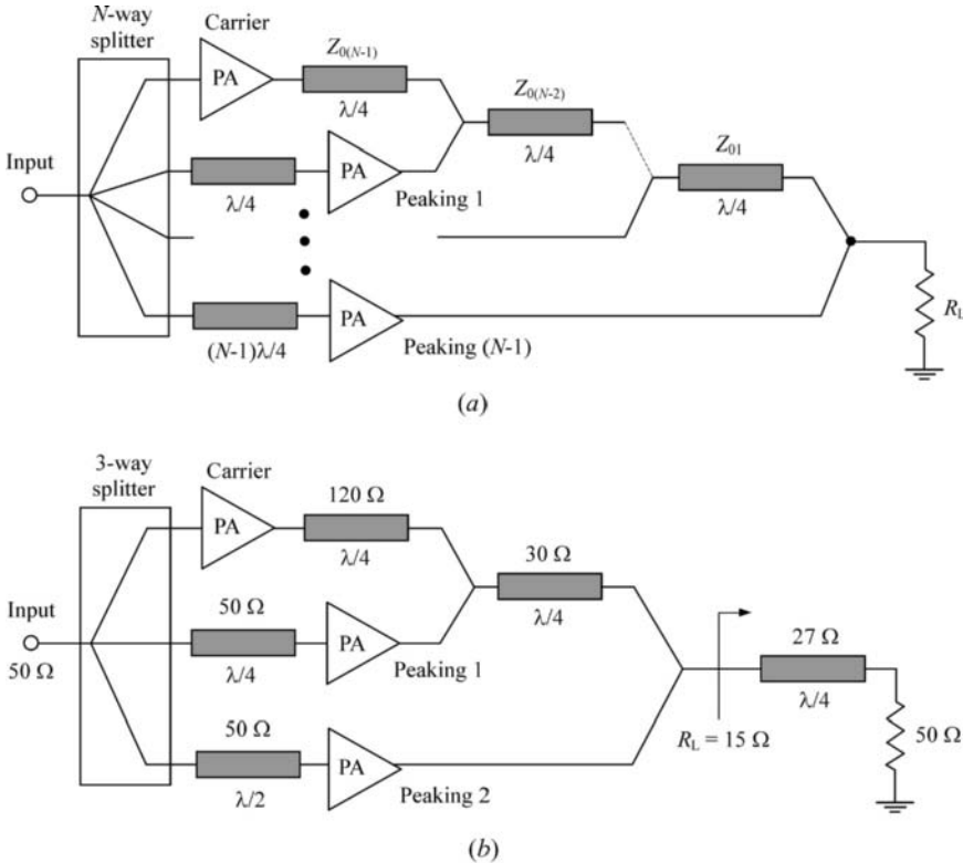
FIGURE 12.24 Multistage Doherty power amplifier architectures.
