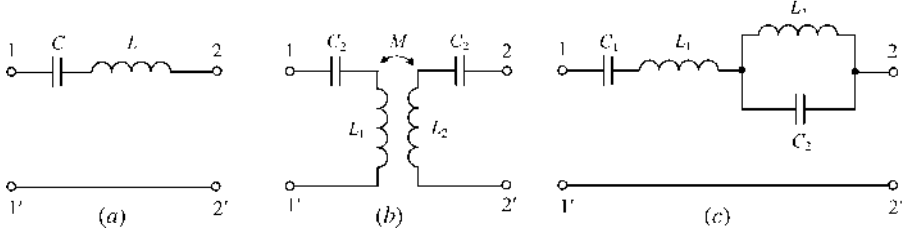
FIGURE 8.50 Schematics of two-port networks.
