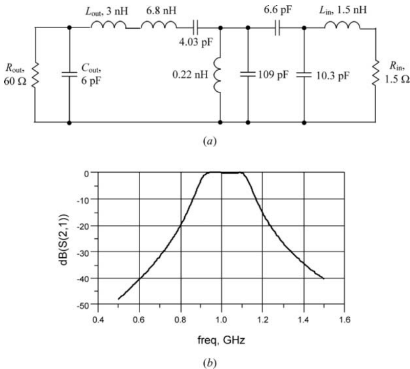
FIGURE 10.47 Impedance-transforming bandpass filter and its frequency response.
