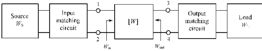
FIGURE 10.1 Generalized single-stage power amplifier circuit.
