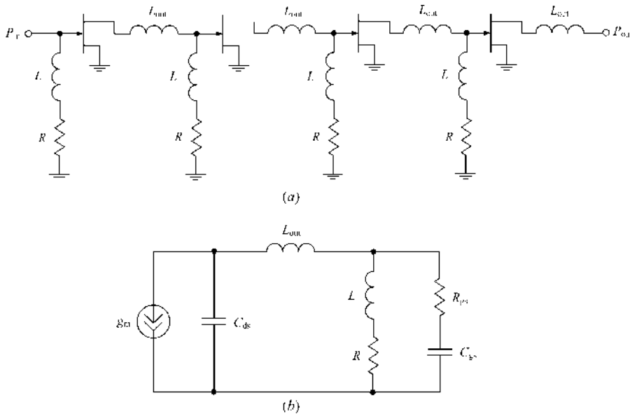
FIGURE 10.52 Schematic of 1–10 GHz four-stage broadband power amplifier.
