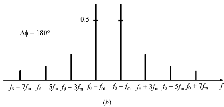
FIGURE 6.35 Binary modulating signal, BPSK signal, and spectrum.
