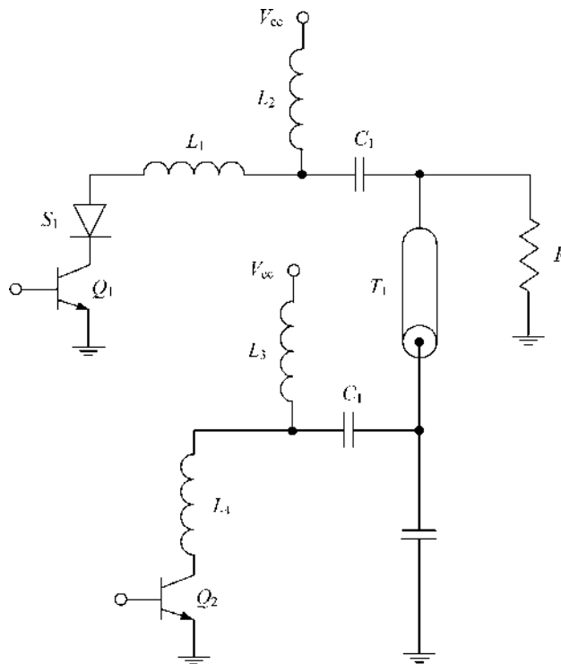
FIGURE 12.40 Switchable path power amplifier circuit.
