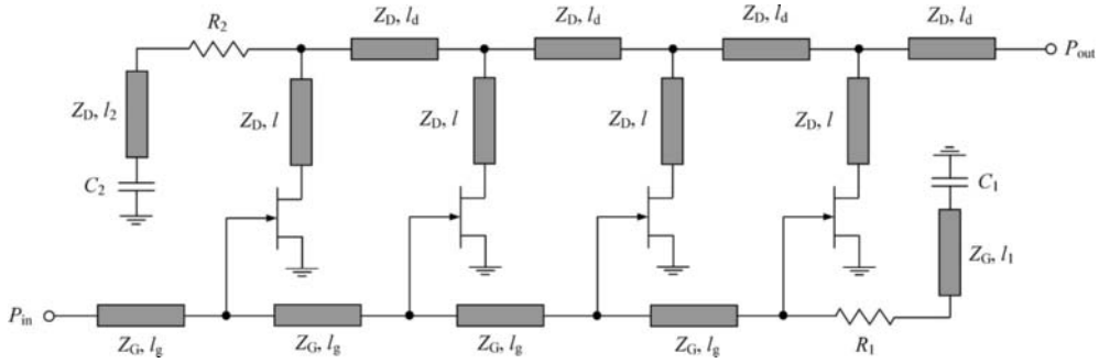
FIGURE 10.55 Schematic representation of four-stage FET traveling-wave amplifier.
