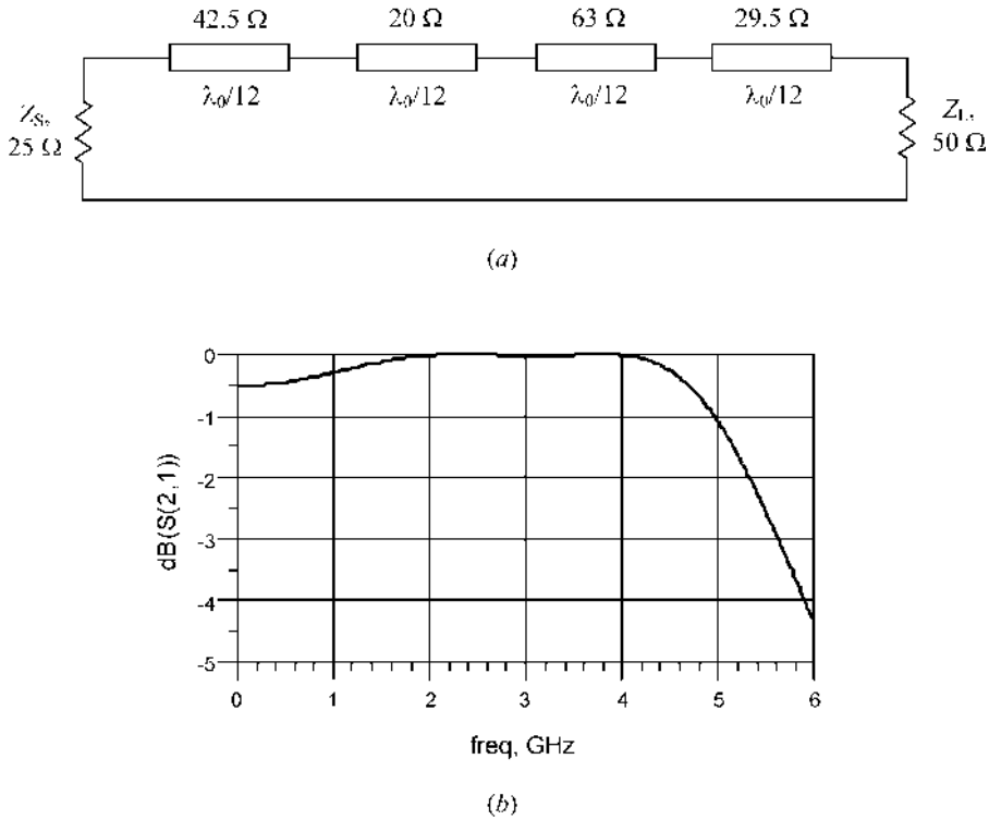
FIGURE 10.48 Stepped transmission-line transformer with equal-length sections.
