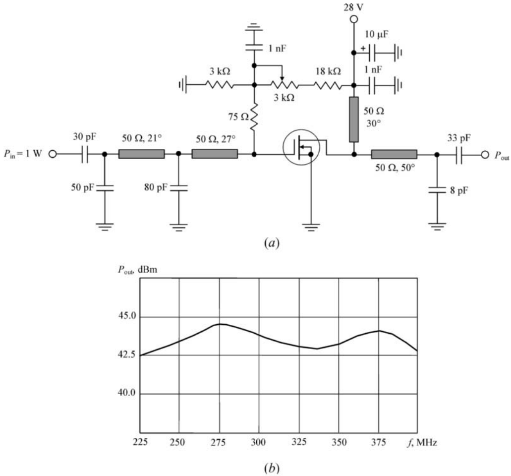
FIGURE 3.40 Circuit schematic and performance of broadband LDMOSFET power amplifier.
