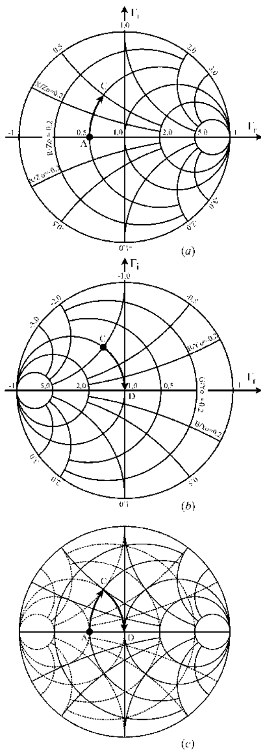
FIGURE 3.3 Simplified impedance and admittance smith charts.
