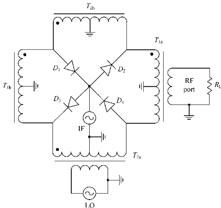
FIGURE 7.9 Schematic of diode double-balanced star mixer.
