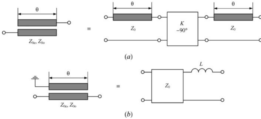
FIGURE 5.24 Equivalent circuits of coupled-line sections.
