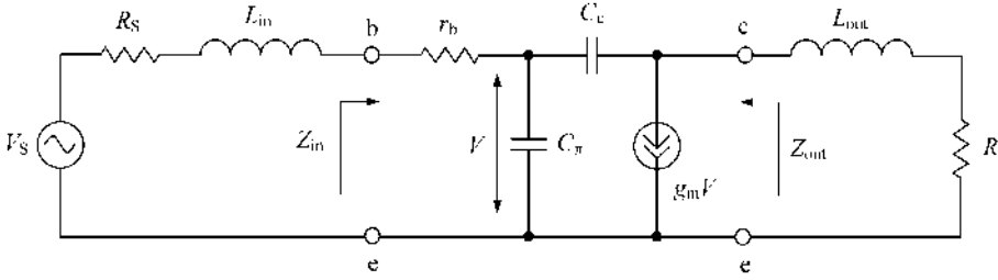
FIGURE 10.2 Simplified equivalent circuit of matched bipolar power amplifier.
