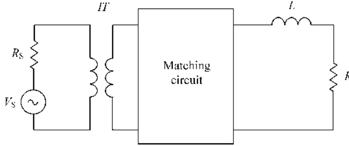
FIGURE 10.40 Matching circuit with ideal transformer.
