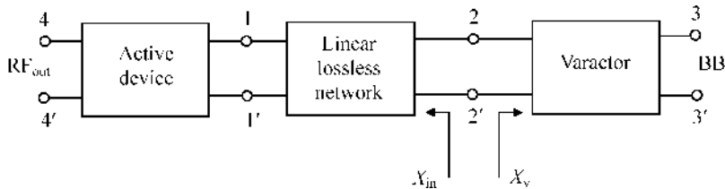
FIGURE 8.48 Block diagram of VCO with linear circuit.
