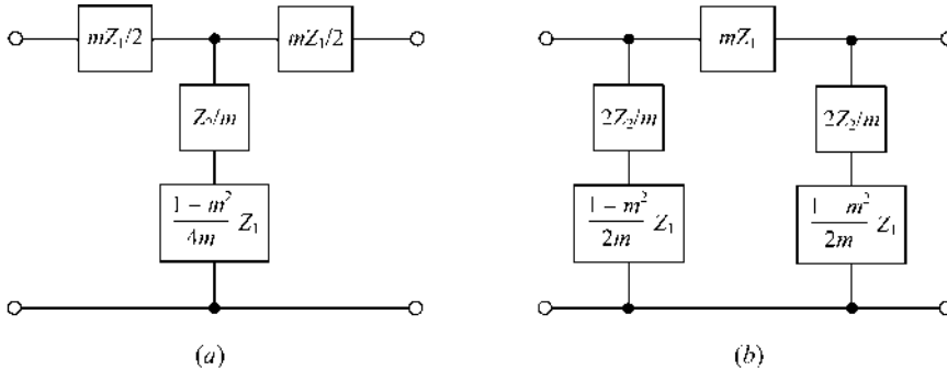
FIGURE 5.7 m -derived filter sections.
