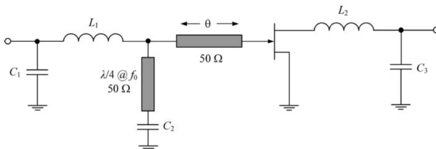
FIGURE 10.64 Circuit schematic of Class AB power amplifier with source harmonic tuning.
