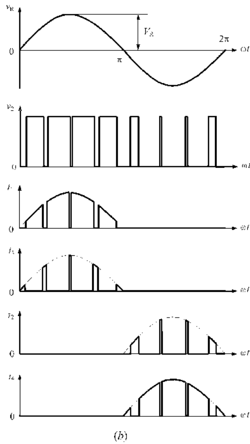
FIGURE 12.50 Class S amplifier with voltage and current waveforms.
