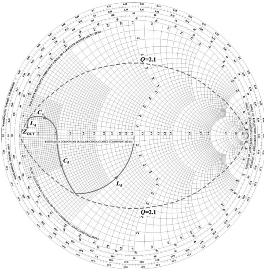
FIGURE 3.25 Smith chart with elements from Figure 3.24.
