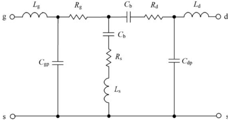
FIGURE 2.23 Small-signal FET circuit at zero drain bias voltage.
