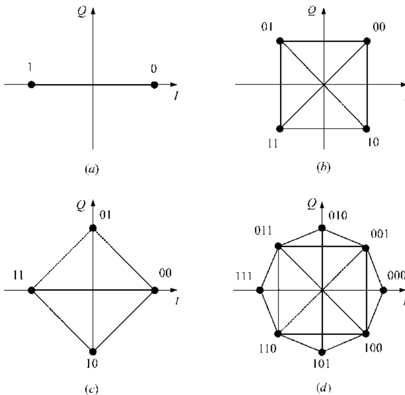
FIGURE 6.37 Trajectories for (a) BPSK, (b) QPSK, (c) shifted QPSK, (d) 8PSK.
