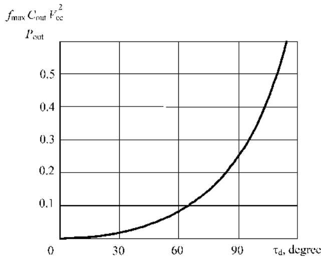
FIGURE 11.59 Normalized maximum operating frequency versus dead time.
