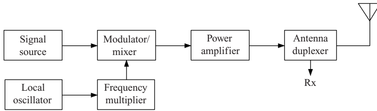
FIGURE I.1 Conventional transmitter architecture.
