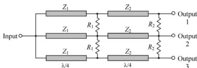
FIGURE 4.26 Microstrip three-way divider with improved isolation.
