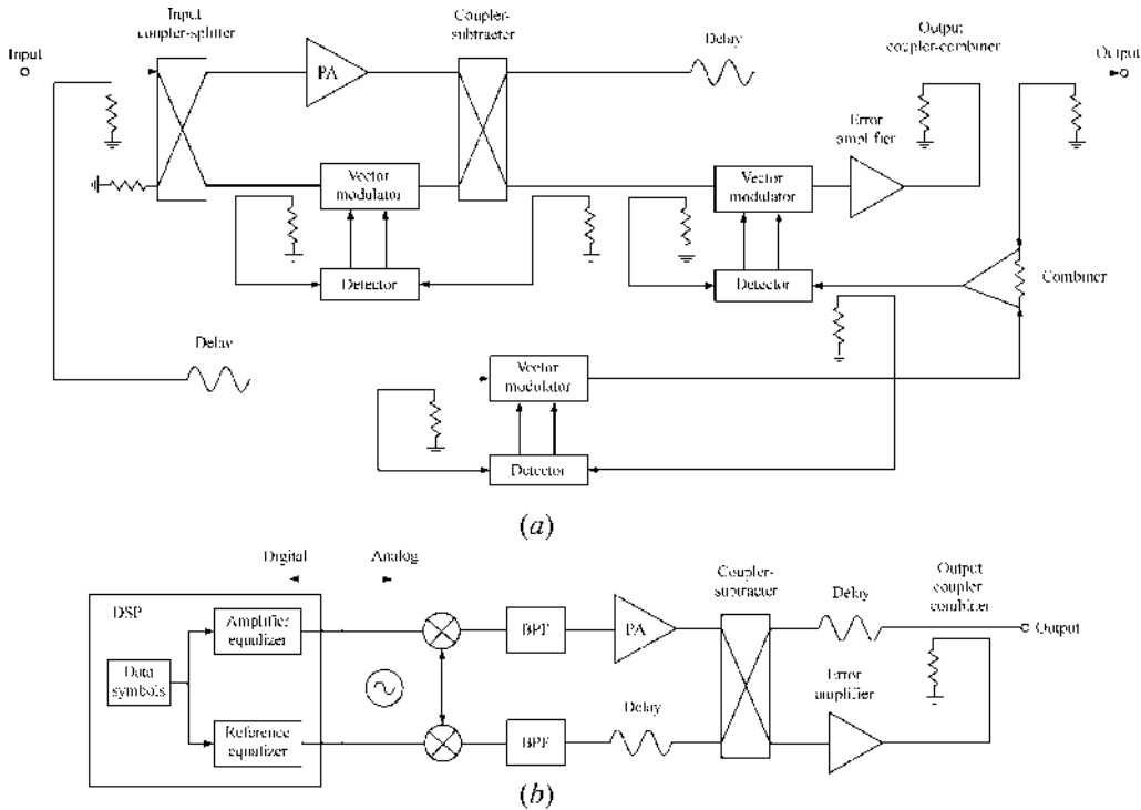
FIGURE 12.4 Adaptive analog and digital feedforward amplifier linearizers.
