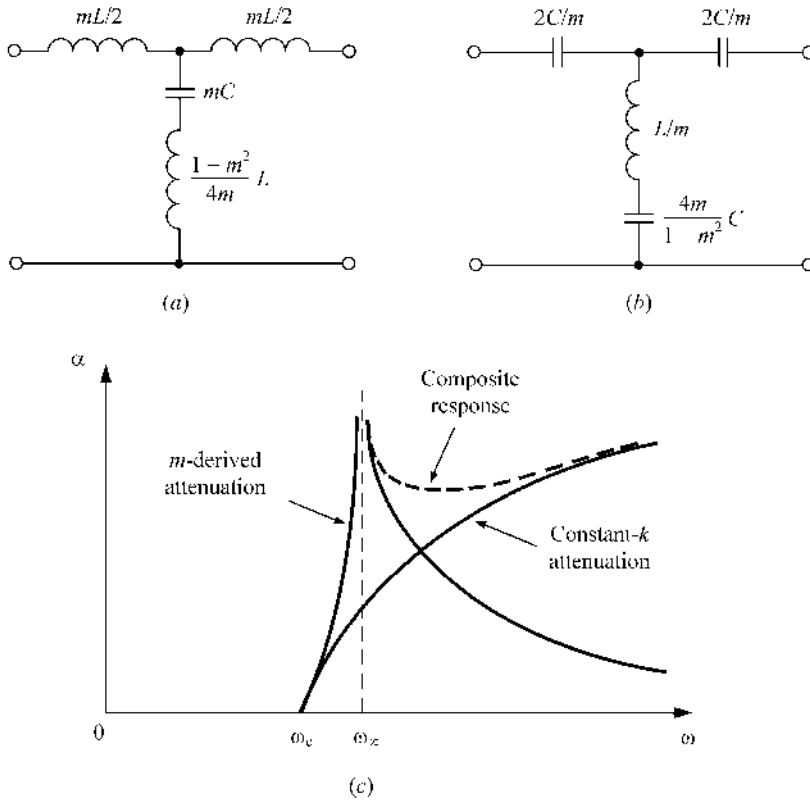
FIGURE 5.8 Low-pass and high-pass m -derived T -sections and frequency response.
