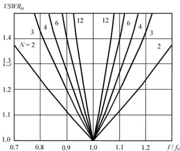
FIGURE 4.22 Frequency performance of N -way Wilkinson divider.
