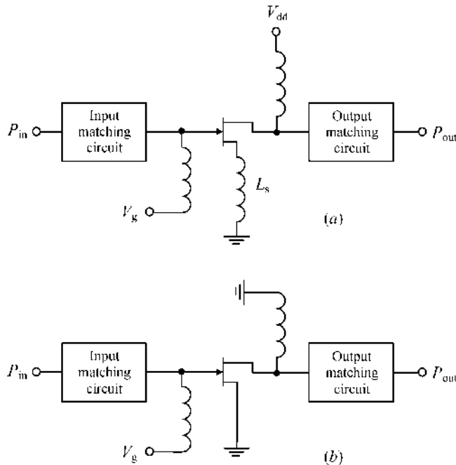
FIGURE 12.9 Transistor-based linearizers.
