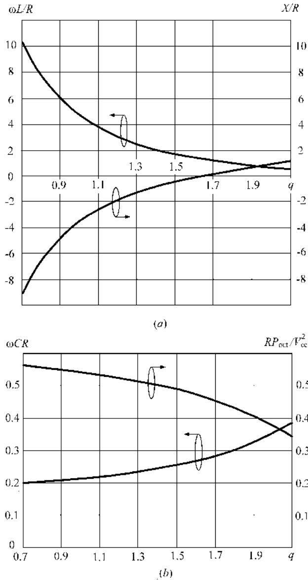
FIGURE 11.49 Normalized optimum quarterwave-line Class E load network parameters.
