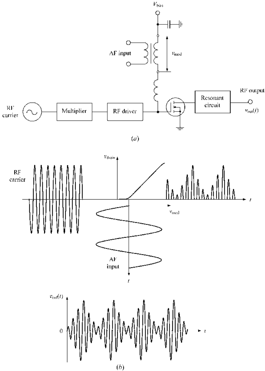
FIGURE 14.4 Basic transmitter structure and operation waveforms for base modulation.
