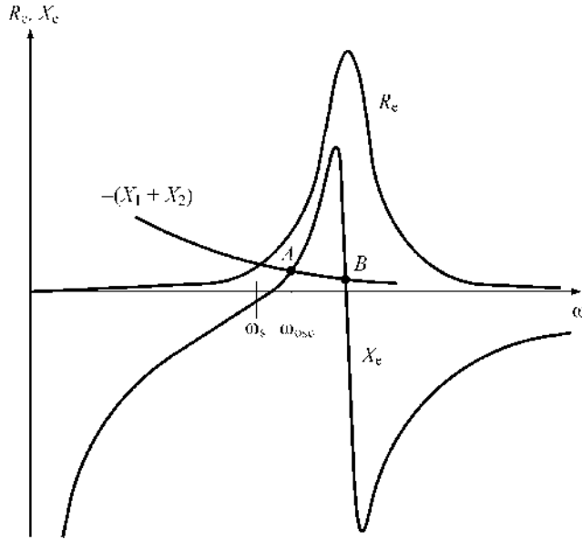
FIGURE 8.61 Resistive and reactive parts of crystal resonator network.
