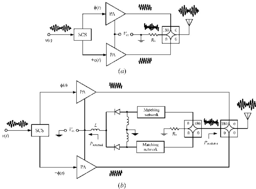
FIGURE 12.31 Outphasing power amplifier system with hybrid combiner.
