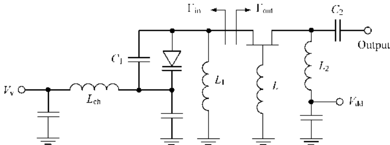
FIGURE 8.51 Circuit schematic of common gate MESFET VCO.
