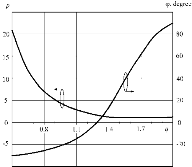
FIGURE 11.37 Optimum Class E parameters p and \varphi versus q .
