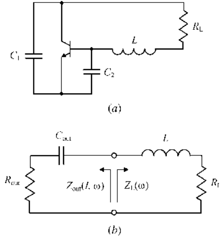
FIGURE 8.27 Parallel feedback (a) electrical and (b) equivalent oscillator circuits.
