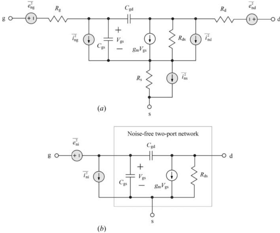
FIGURE 2.18 MOSFET equivalent circuits with noise sources.
