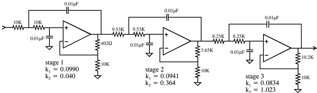
FIGURE 3-9 A six pole Bessel filter formed by cascading three Sallen-Key circuits. This is a low-pass filter with a cutoff frequency of 1 kHz.
