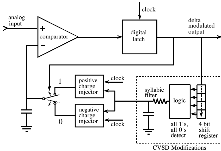
FIGURE 3-18 CVSD modulation block diagram. A logic circuit is added to the basic delta modulator to improve the slew rate.
